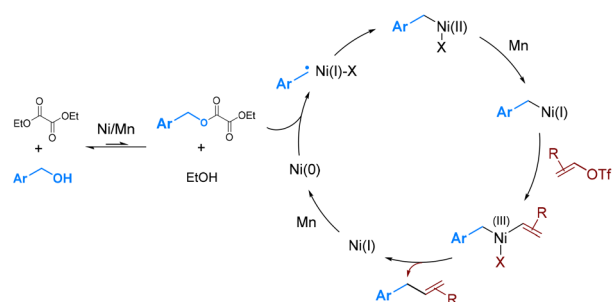
Scheme 5 Proposed mechanism.
