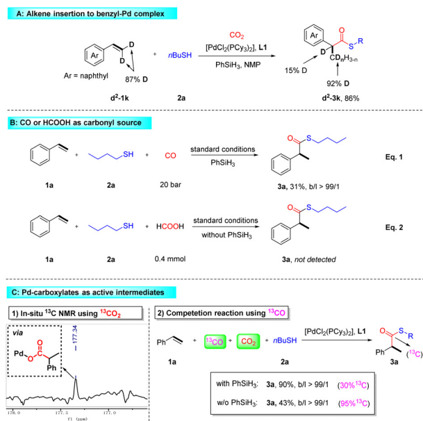
Scheme 4 Experimental studies on the mechanism. Reaction conditions: 1a / d 2 -1k (0.2 mmol), 2a (1.7 equiv.), PdCl_2(PCy_3)_2 (5.0 mol%), L1 (10.0 mol%), PhSiH_3 (1.8 equiv.), CO_2 (20 bar), NMP (0.5 mL), and stirred at 80 °C for 18 h. Isolated yields of branched products.
