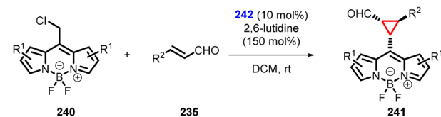
Scheme 54 MIRC cyclization to synthesize cyclopropane carbaldehydes derived from BODIPY.
