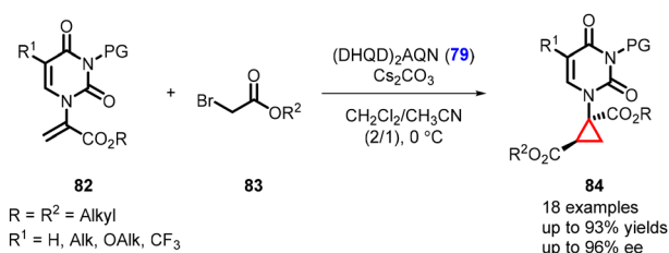
Scheme 15 Enantioselective cyclopropanation of \alpha -pyrimidine substituted acrylates.
