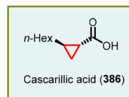
Scheme 85 MIRC cyclopropanation of 4-chloro- \alpha,\beta -unsaturated esters/thioesters/ketones with Grignard reagents.
