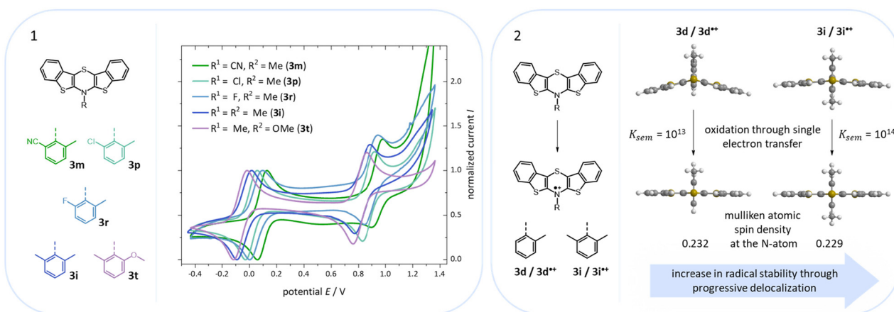
Fig. 8 (1) CVs of BBTs of 3m , 3p , 3r , 3i , and 3t (CVs recorded in CH 2 Cl 2 , T = 298 K, 0.1 M [ n Bu 4 N][PF 6 ], \nu = 100 mV s -1 , Pt-working- und counter electrode, Ag/AgCl(3 M)-reference electrode, referenced with decamethylferrocene (DMFc)/DMFc + , potential vs. Fc/Fc + = 0.00 V). (2) Minimum geometries of BBTs 3d and 3i as well as their corresponding radical cations 3d •+ and 3i •+ ((u)B3LYP/6-311++G**, IEFPCM CH 2 Cl 2 ) and illustration of the increase in the radical stability.
