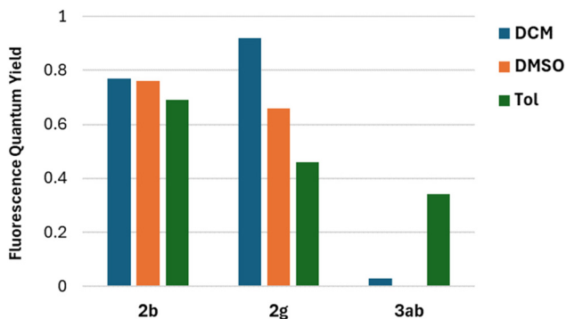
Fig. 3 Comparison of Fluorescence quantum yield in different solvents for representative compounds 2b , 2g and 3ab .
