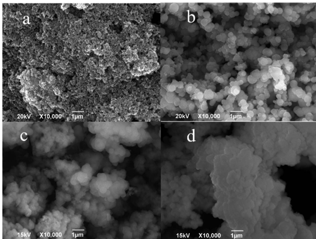
Fig. 4 SEM images of (a) \text{CoFe}_2\text{O}_4 , (b) \text{CoFe}_2\text{O}_4@SiO_2 , (c) \text{CoFe}_2\text{O}_4@SiO_2-NH_2 and (d) \text{CoFe}_2\text{O}_4@SiO_2-NH_2 nanoparticles after adsorption of lead ions.
