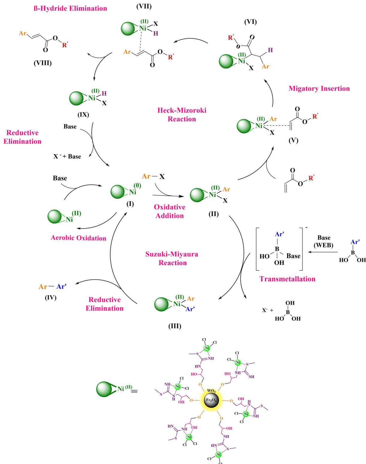
Scheme 4 Proposed catalytic mechanism of the Heck–Mizoroki and Suzuki–Miyaura reactions catalysed by the \text{Fe}_3\text{O}_4 @ \text{WO}_3 -E-SMTU- \text{Ni}^{II} nanostructured catalyst.
