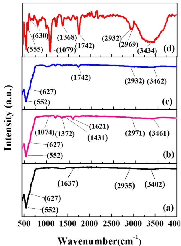
Fig. 2 ATR-FTIR spectra of (a) MIONPs, (b) CS/MIONPs, (c) GA/CS/MIONPs and (d) Urease/GA/CS/MIONPs.
