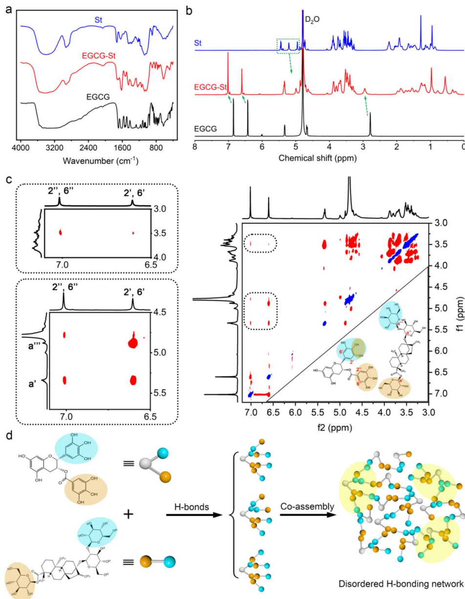
Fig. 3 (a) FT-IR spectra of EGCG, St, and EGCG–St hydrogel, (b) ^1\text{H} NMR spectra of EGCG, St, and EGCG–St mixture in \text{D}_2\text{O} , (c) 2D ROESY NMR spectrum (600 MHz) of EGCG–St mixture, and (d) the proposed co-assembly mode for the EGCG–St hydrogel.
