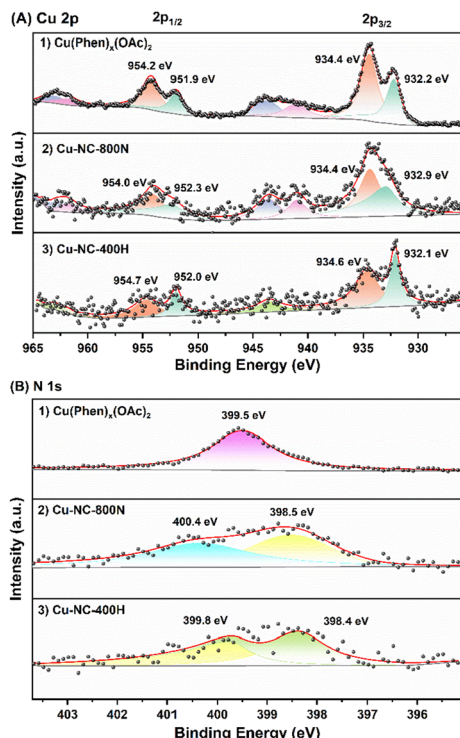
Fig. 5 The XPS of (A) Cu 2p signals: (1) \text{Cu}(\text{Phen})_x(\text{OAc})_2 , (2) Cu-NC-800N, and (3) Cu-NC-400H samples and (B) N 1s signals: (1) \text{Cu}(\text{Phen})_x(\text{OAc})_2 , (2) Cu-NC-800N, and (3) Cu-NC-400H samples.
