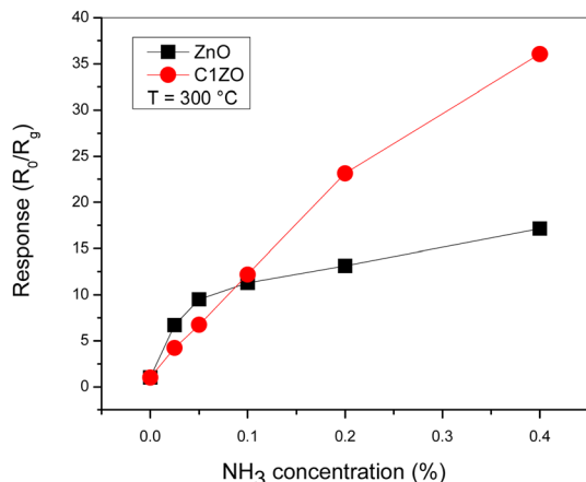
Fig. 8 Comparison between pure ZnO and ZnO:Ca 1% sensors response toward different NH 3 concentrations at T = 300 °C.
