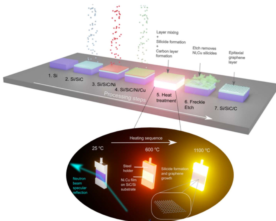
Fig. 1 Schematic of the Ni/Cu catalytic alloy-mediated EG synthesis on 3C-SiC on silicon.
