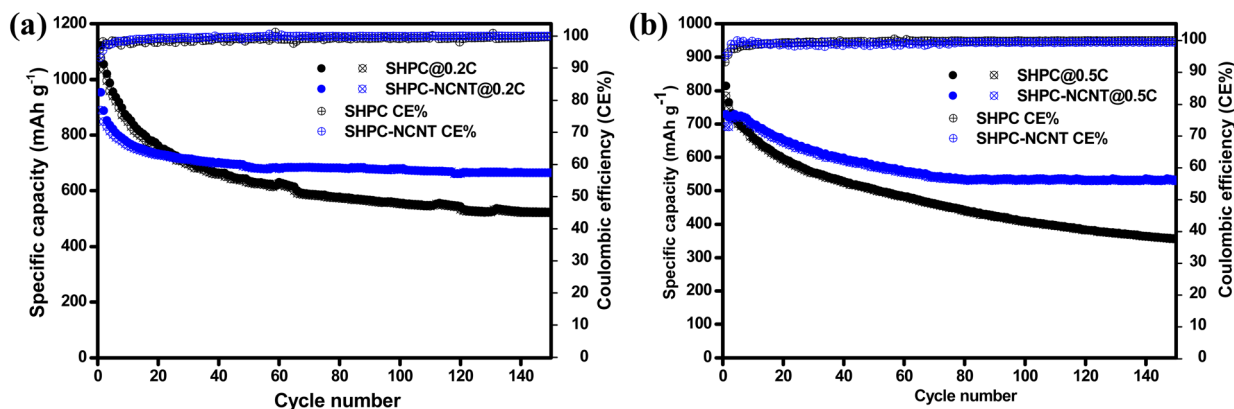
Fig. 8 Cyclability with coulombic efficiency results of SHPC and SHPC-NCNTs composite at (a) 0.2C rate (b) 0.5 rate.
