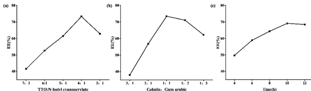
Fig. 2 Effects of ratio of TTO to n -butyl cyanoacrylate (a), mass ratio of gelatin to gum arabic (b) and curing time (c) on EE.
