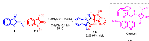
Scheme 38 Synthesis of 3,2'-pyrrolidiny bispriooxindoles from 3-isothiocyanato oxindoles and \alpha,\beta -unsaturated ketones.
