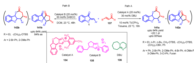
Scheme 45 Stereoselective synthesis of \epsilon -lactones or spiro-heterocycles through NHC-catalysed annulation.
