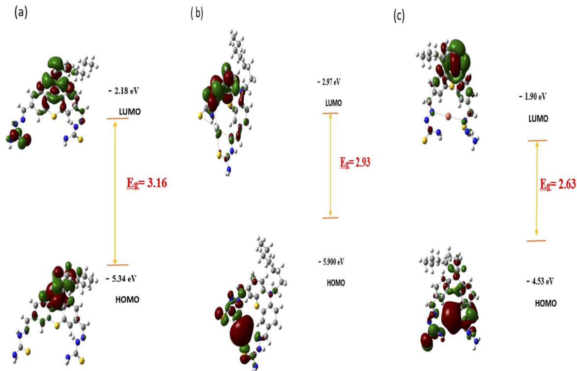
Fig. 4 HOMO, LUMOs, and bandgaps of (a) PTZDS, (b) PTZDS + Hg 2+ and (c) PTZDS + Cu 2+ .
