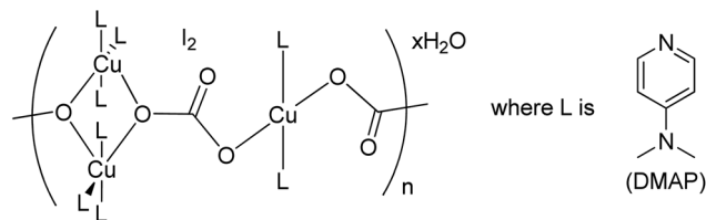
Fig. 2 Structure of the \mu_3 -CO 3 bridged linear polymeric Cu-complex ((Cu 3 (DMAP) 8 (CO 3 ) 2 ) n ·xH 2 O).
