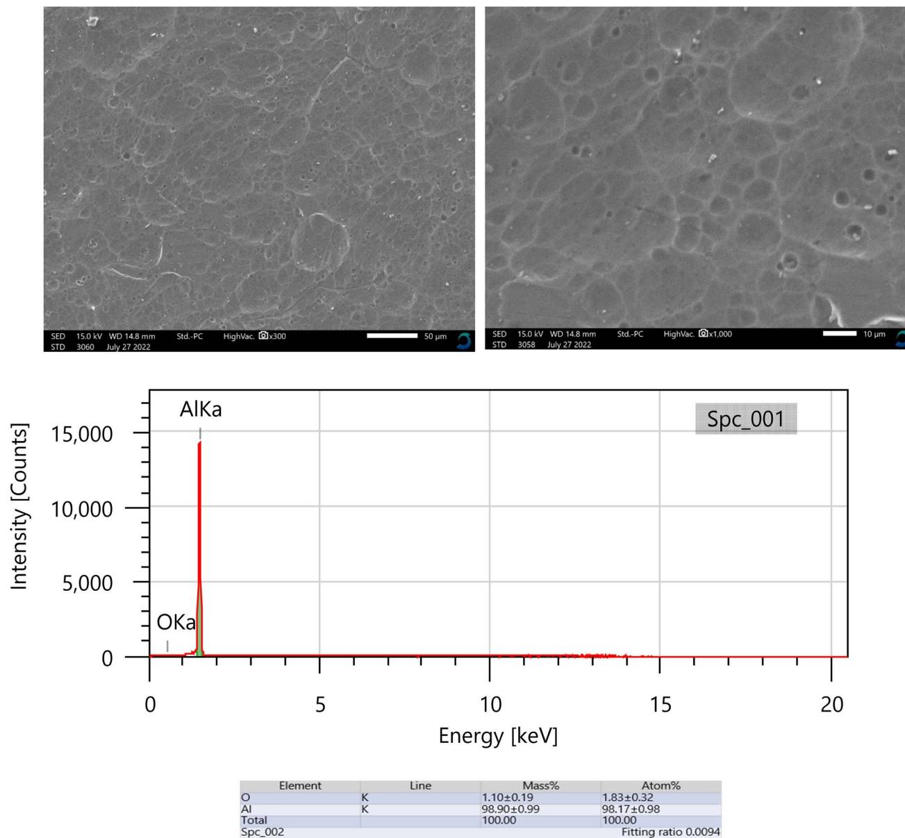
Fig. 6 SEM/EDX for Al after immersion 0.5 M NaOH in the presence of 0.01 M of isopropinosine inhibitor.
