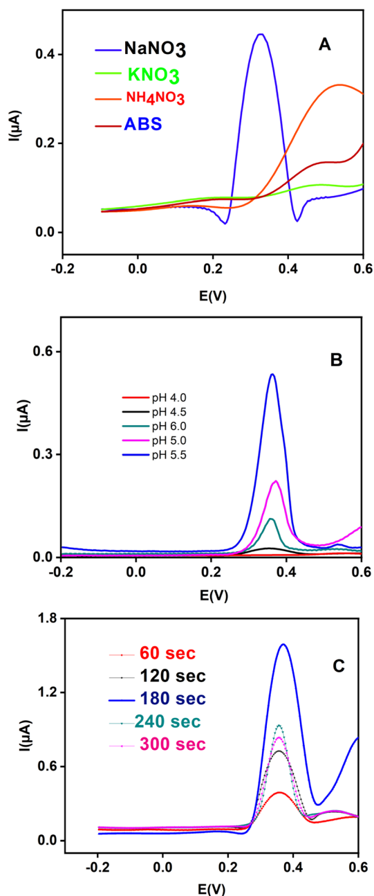
Fig. 8 Determination of Hg(II) via square wave anodic stripping voltammetry using SDA/MWCNTs at 55 \mu\text{g per L Hg(II)} in (A) different electrolytes, (B) pH media, and (C) preconcentration time with various time intervals at a scan rate of 50 \text{ mV s}^{-1} .
