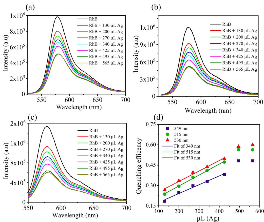
Fig. 6 Fluorescence spectra of RhB (1.2 \mu M) in comparison with the mixtures of Ag nanodisks + RhB (1.2 \mu M), with the amount of stock Ag nanodisks varying from 130 \mu L to 565 \mu L in a titration volume of 1700 \mu L, under different excitation wavelengths at 349 nm (a), 515 nm (b), and 530 nm (c); (d) fluorescence quenching efficiency of mixed solutions of Ag nanodisks + RhB depending on the amount of stock Ag nanodisks solution and the excitation wavelength.
