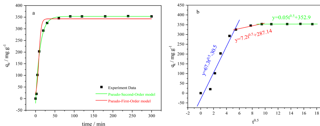
Fig. 4 Adsorption capacity of BC-CLS under different contact times, the corresponding pseudo-first-order, pseudo-second-order kinetics (a) and intra-particle diffusion model (experiment condition: adsorbent dose 0.01 g, temperature 298 K, pH 5, time 5–300 min, concentration 100\text{ mg g}^{-1} , solution volume 50 mL).
