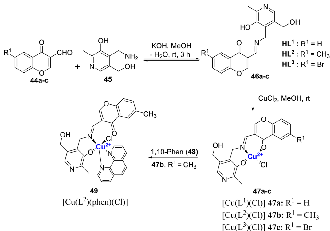
Scheme 12 Synthesis of ligands 46a–c and their complexation with Cu 2+ ions 47a–c and 49.
