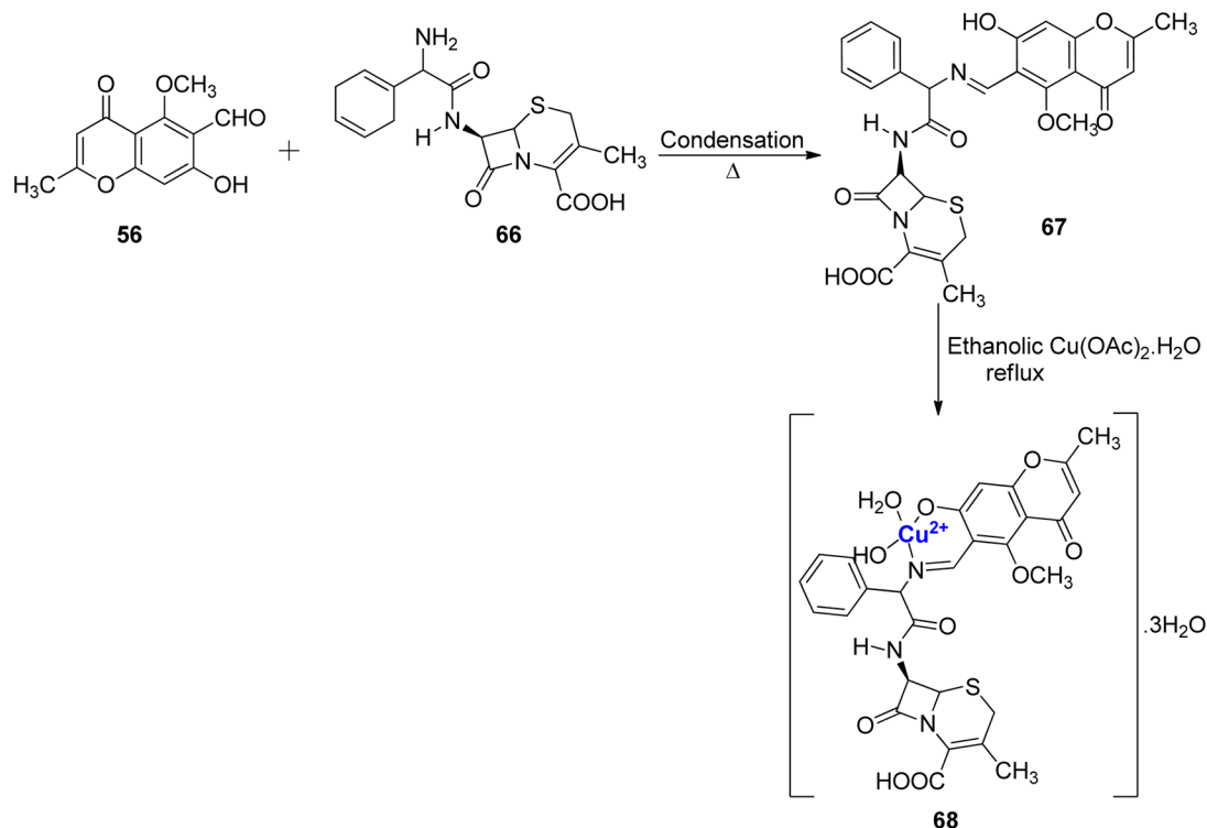
Scheme 18 Synthesis of ligand 67 and its complexation with Cu 2+ ions to give 68 .
