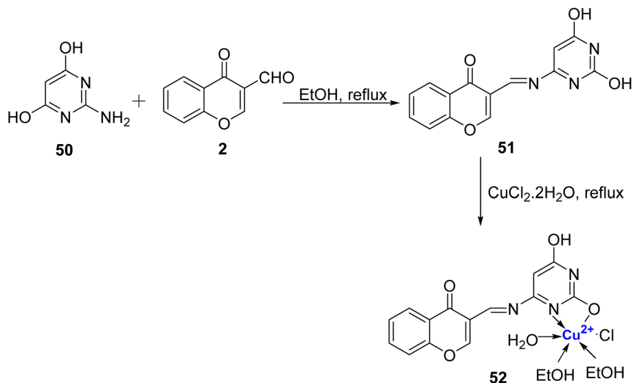
Scheme 13 Synthesis of ligand 51 and its Cu(II)-complex 52 .
