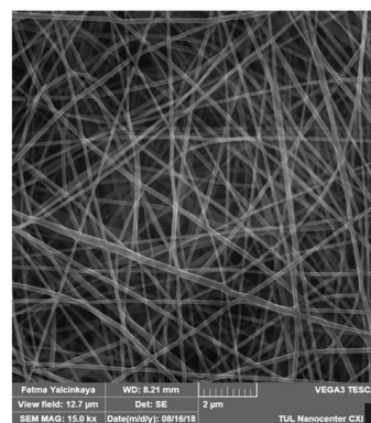
Fig. 3 Polymeric polyamide 6 nanofibers with an average fiber diameter 114 \pm 22 \text{ nm} .
