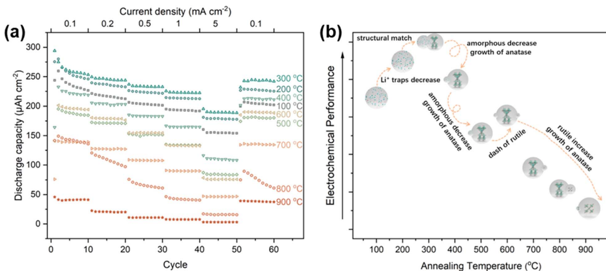
Fig. 7 (a) High rate cycling performance of TNTAs grown for 2 h and annealing at different temperatures. Current density is 0.1–5 mA \text{cm}^{-2} . (b) Relationship between electrochemical properties and annealing temperature.
