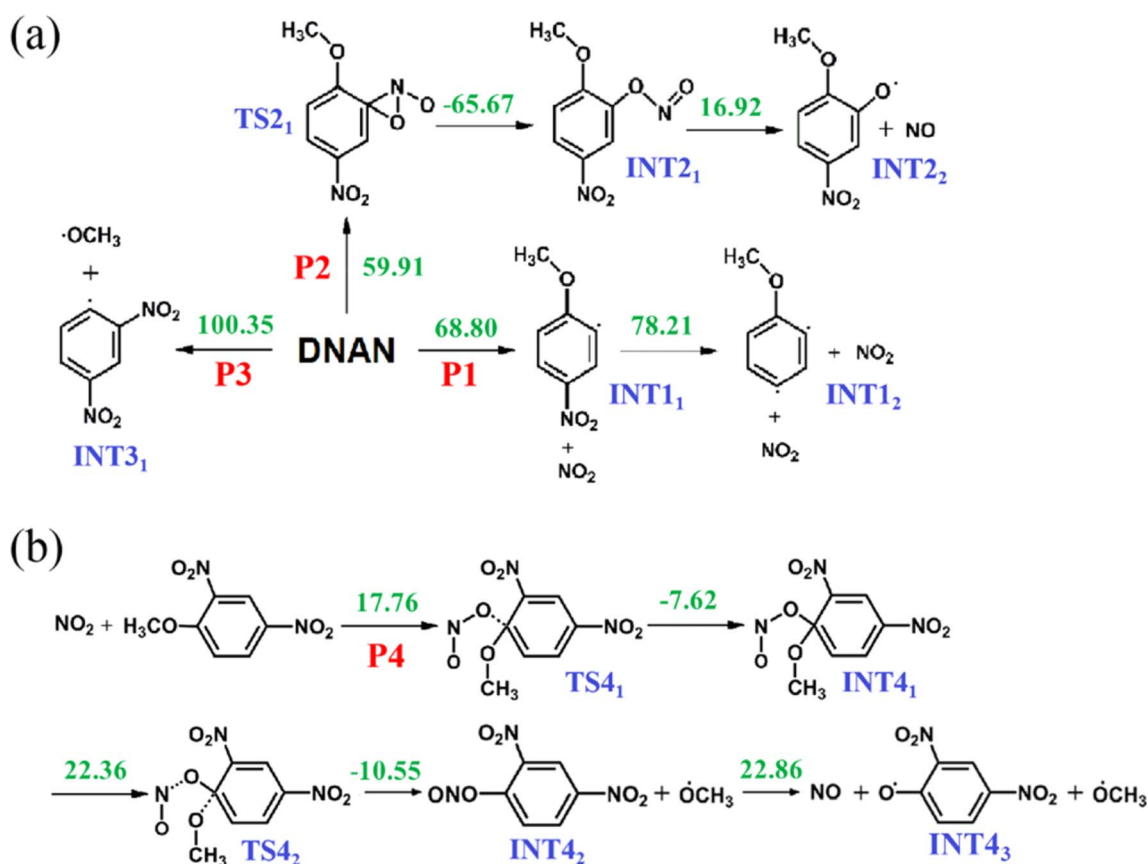
Fig. 5 (a) Major unimolecular reaction paths (P1 to P3) and (b) bimolecular reaction path (P4) during the decomposition of the DNAN. Numbers in green are enthalpy changes of each step at 500 K (kcal mol -1 ) calculated from DFT.
