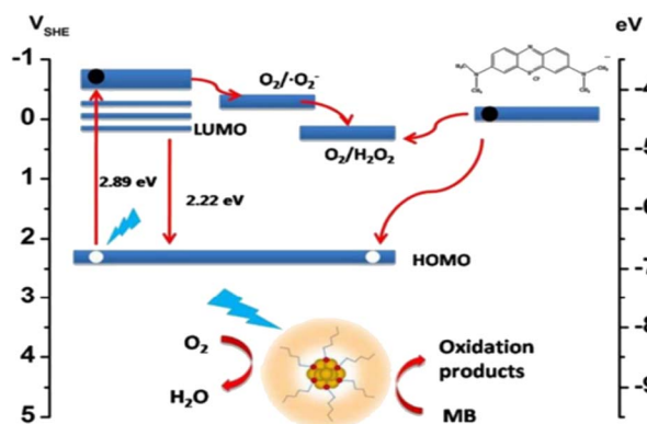
Fig. 8 Mechanism of the degradation of MB dye. Reproduced with permission from ref. 150, copyright 2024, Nanoscale.
