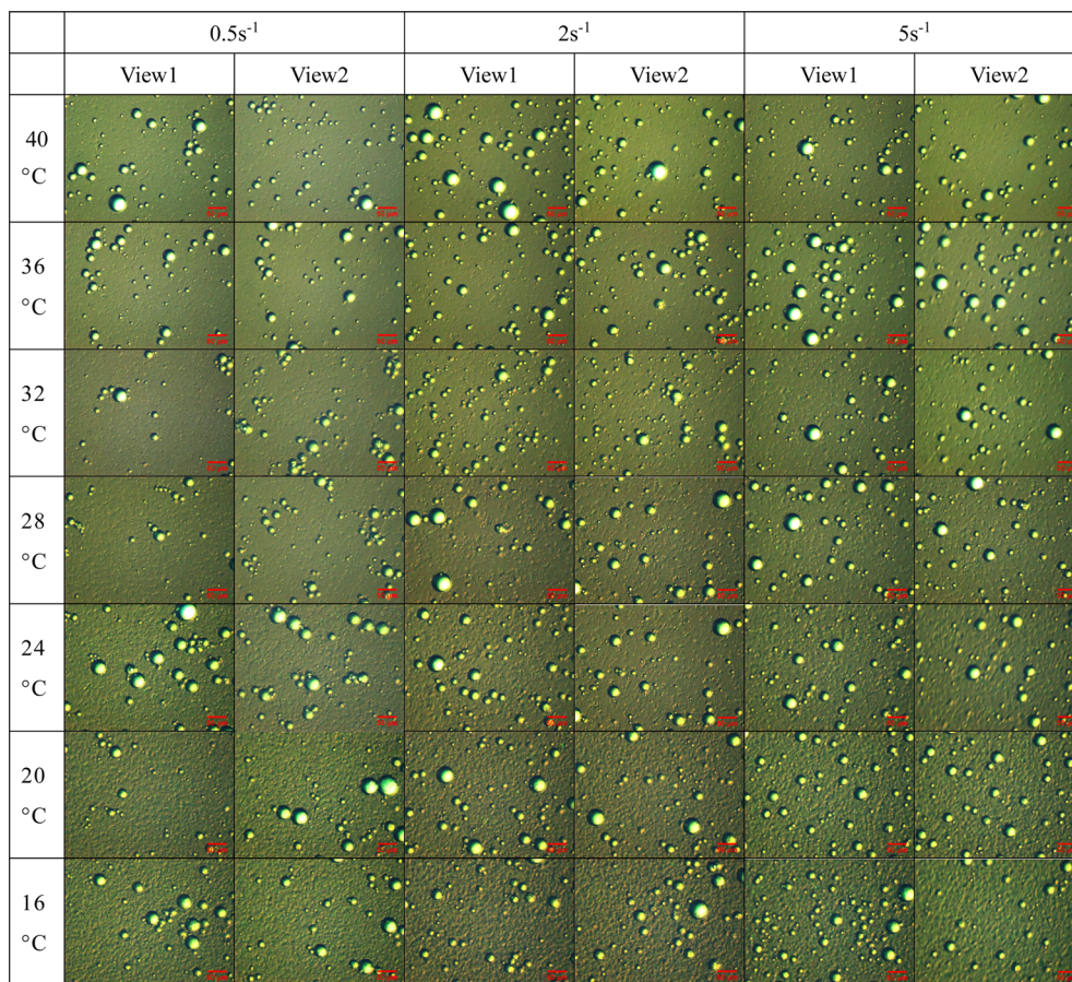
Fig. 2 Microscopic images at different shear rates during cooling (scale bar: 50 μm).
