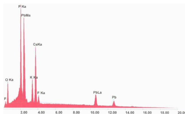
Fig. 1 Energy-dispersive X-ray spectrum of KPbFAP .
