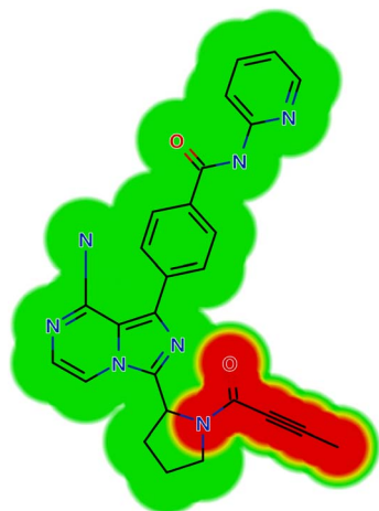
Fig. 5 Structural alerts of acalabrutinib by DEREK module (skin sensitization; equivoal).
