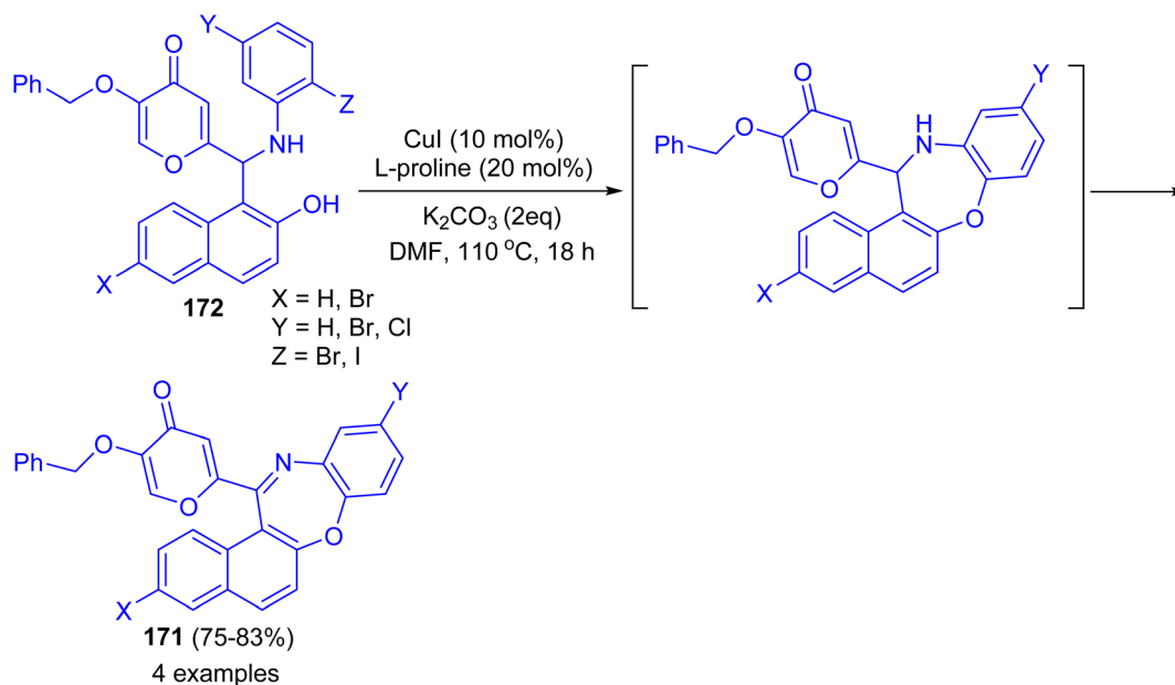
Scheme 48 Synthesis of oxazepine derivatives 171 .
