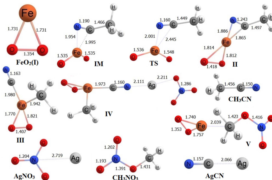
Fig. 3 Optimized geometries of all species at \omega\text{B97XD}/6\text{-}311++\text{G}(\text{d},\text{p})/\text{LANL2DZ} level of theory.
