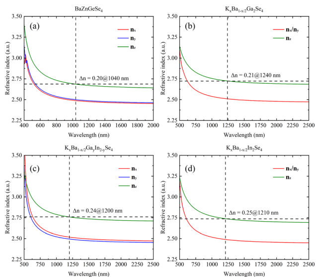
Fig. 7 (a)–(d) The linear optical properties of \text{BaZnGeSe}_4 , \text{K}_x\text{Ba}_{1-x/2}\text{Ga}_2\text{In}_{2-y}\text{Se}_4 , \text{K}_x\text{Ba}_{1-x/2}\text{Ga}_2\text{In}_{2-y}\text{Se}_4 , and \text{K}_x\text{Ba}_{1-x/2}\text{In}_2\text{Se}_4 .
