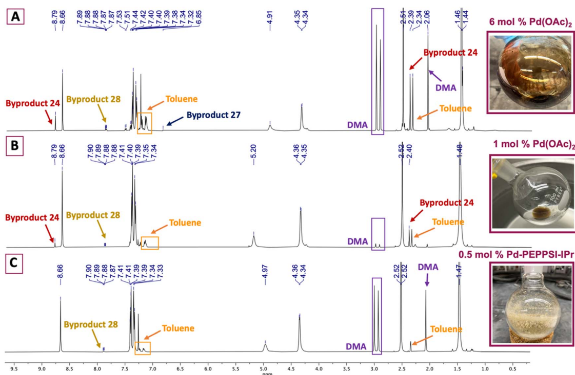
Fig. 2 1 H NMR and photographic comparison of crude 10 formed using: (A) 6 mol% Pd(OAc) 2 ; (B) 1 mol% Pd(OAc) 2 ; (C) 0.5 mol% Pd-PEPPSI-IPr. Residual reaction solvent, DMA, and azeotropic solvent, toluene, are indicated.
