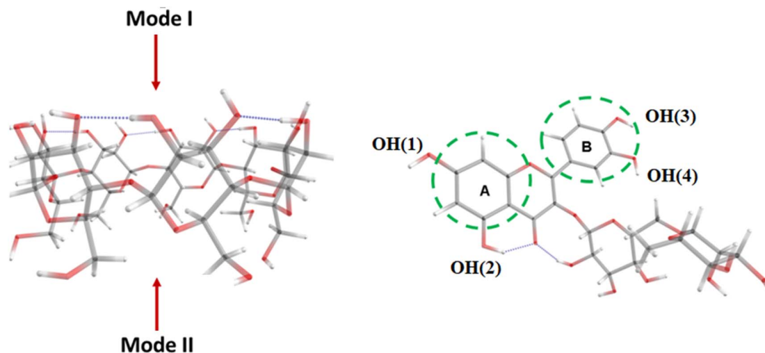
Fig. 1 Interaction modes between rutin and \beta -CD. Color codes: grey – C, red – O, white – H, and numbering scheme of phenolic –OH groups in Rutin molecule.
