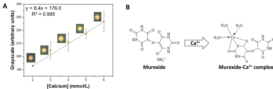
Fig. 3 Detection of calcium in the proposed \mu\text{PAD} . (A) Calibration curve obtained for \text{Ca}^{2+} in concentrations ranging from 2.0 to 6.0 \text{mmol L}^{-1} . (B) Structure of murexide and the murexide- \text{Ca}^{2+} complex.
