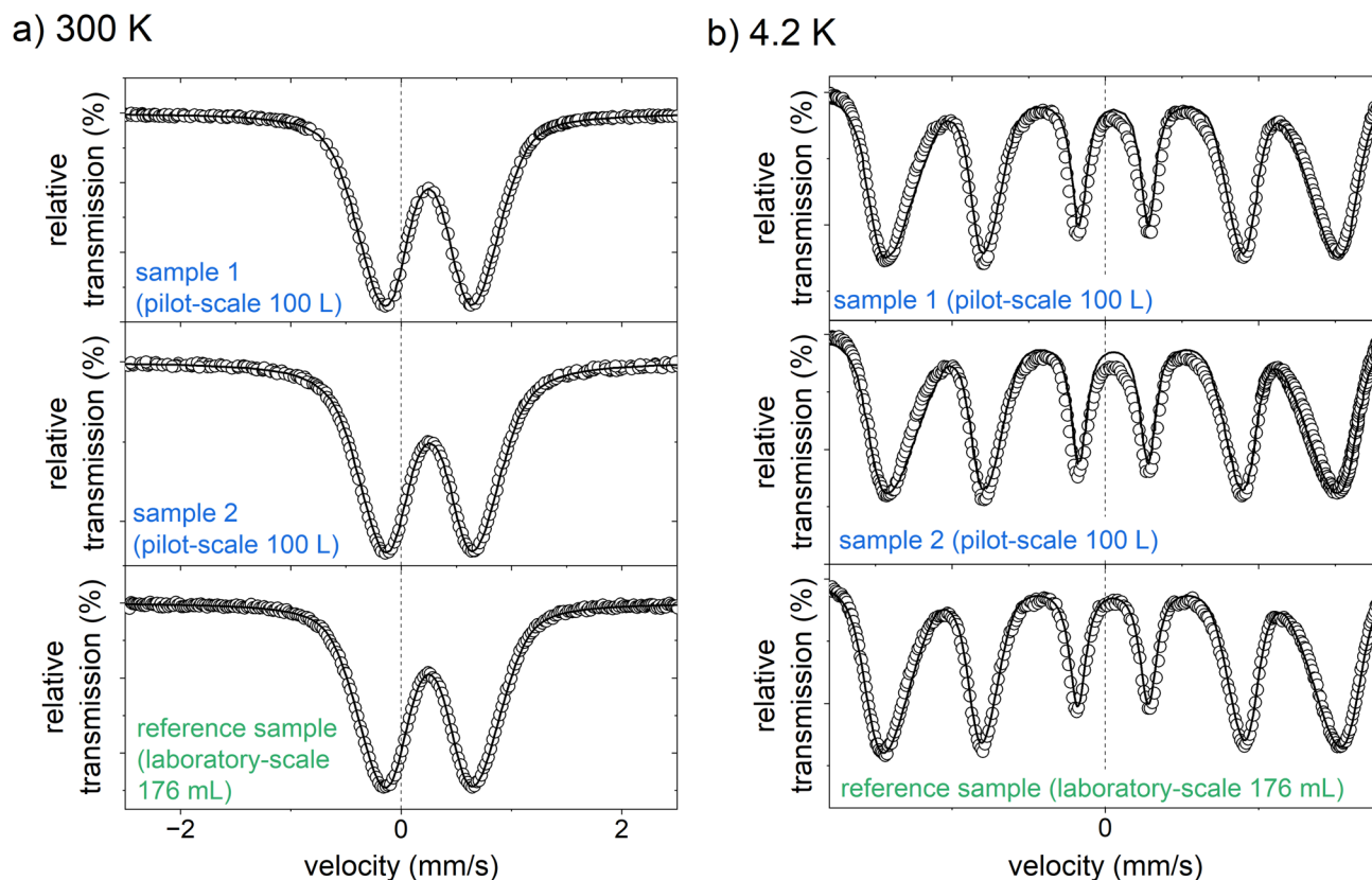
Fig. 5 Mössbauer spectra of the two active ingredient samples prepared on a pilot-scale (100 L), and the reference sample, produced on a laboratory scale (176 mL, data reproduced by Bäumlner et al. 24 ) measured at (a) 300 K, and (b) 4.2 K.
