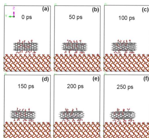
Fig. 7 State of CNT grafted with 10% carboxyl groups on SiO 2 surface at different time. (a) 0 ps; (b) 50 ps; (c) 100 ps; (d) 150 ps; (e) 200 ps; (f) 250 ps.
