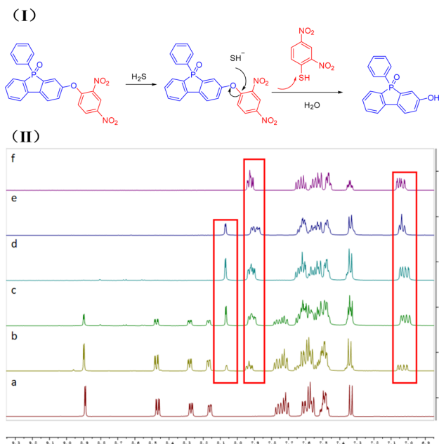
Fig. 6 (I) Possible mechanism for the probe PPF-CDNB with \text{H}_2\text{S} . (II) ^1\text{H-NMR} titration experiments of probe PPF-CDNB. (a) PPF-CDNB. (b) PPF-CDNB + 1 eq. NaHS. (c) PPF-CDNB + 3 eq. NaHS. (d) PPF-CDNB + 5 eq. NaHS. (e) PPF-CDNB + 10 eq. NaHS. (f) PPF-OH. ^1\text{H-NMR} measurements were performed 10 min after addition of NaHS to PPF-CDNB (600 MHz, \text{DMSO-d}_6 ).
