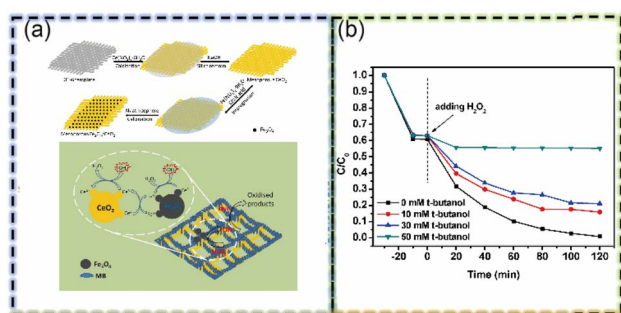
Fig. 10 (a) Schematic diagram for the preparation of mesoporous Fe 3 O 4 /CeO 2 and MB removal mechanism by mesoporous Fe 3 O 4 /CeO 2 composite. (b) Effect of t-butanol on removal of MB in Fe 3 O 4 /CeO 2 (Fe:Ce = 1:1) catalyzed system (this figure has been reproduced with permission from Li et al. 85 from Elsevier, copyright 2017).
