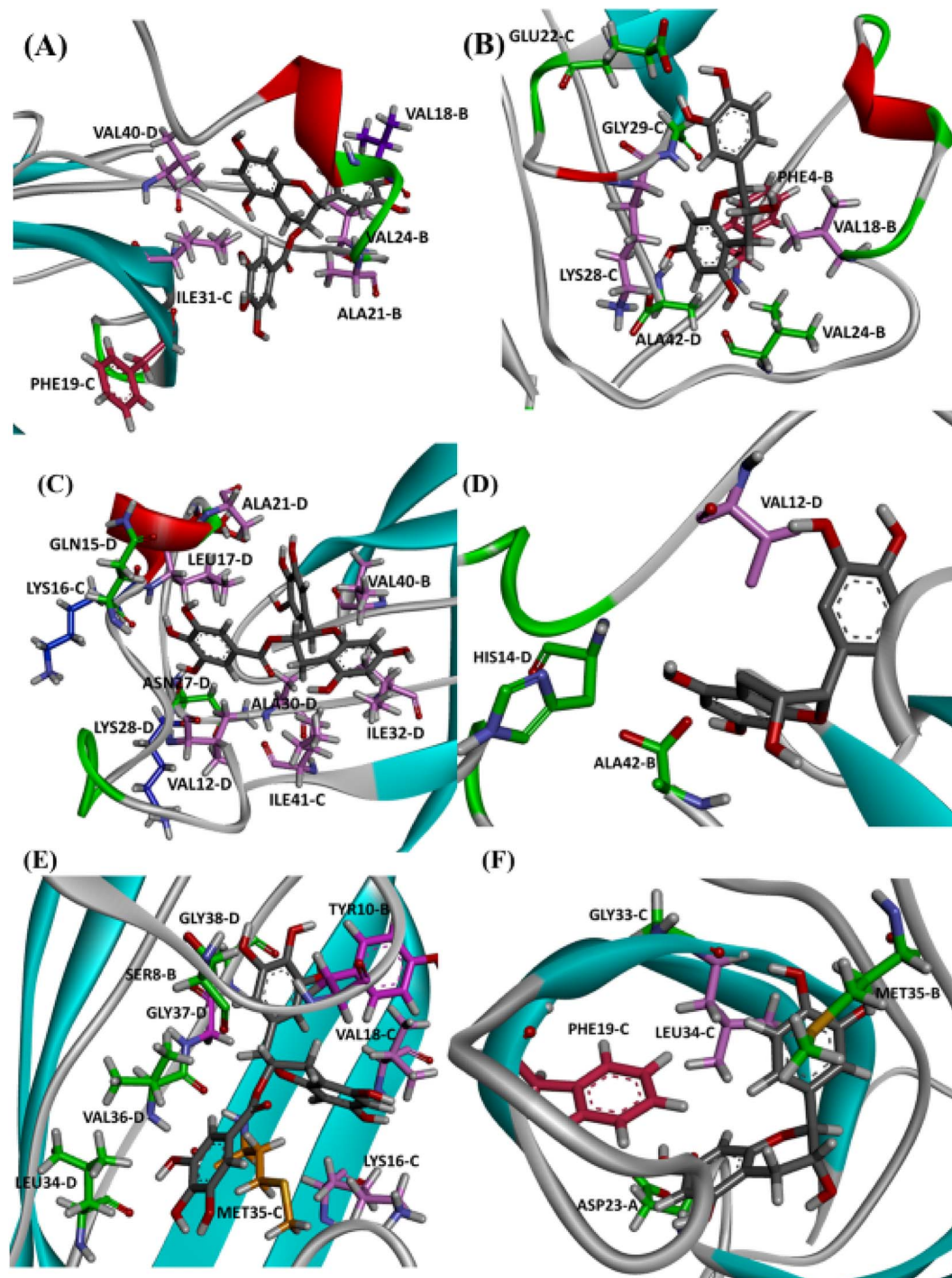
Fig. 8 Intermolecular interactions observed in the final state of complex EGCG- \beta O and EC- \beta O docked in site P0 (A), P1 (B), and P2 (C) for md1. The oligomer structure is shown in cyan, and the ligands are represented as gray sticks. Residues involved in H-bonding are shown as green sticks, while residues involved in electrostatic interactions are represented as light pink ( \pi -alkyl), hot pink ( \pi -stacking), and orange ( \pi -sulfur).
