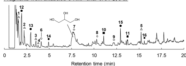
Fig. 5 Pyrogram obtained from the Py-GC/MS analysis (764 °C, 5 s hold time) of 5-HMF char generated by carbonization at 280 °C for 60 min.
