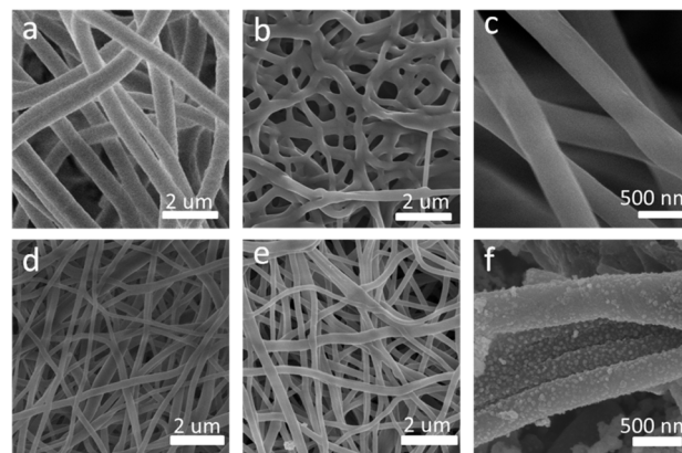
Fig. 2 SEM images of pure PVA fibers (a); carbon nanofibers carbonized at 600 °C for 2 h (b and c); uncarbonized Ni/PVA-based fibers (d); Ni/C nanofibers carbonized at 600 °C for 2 h (e and f).
