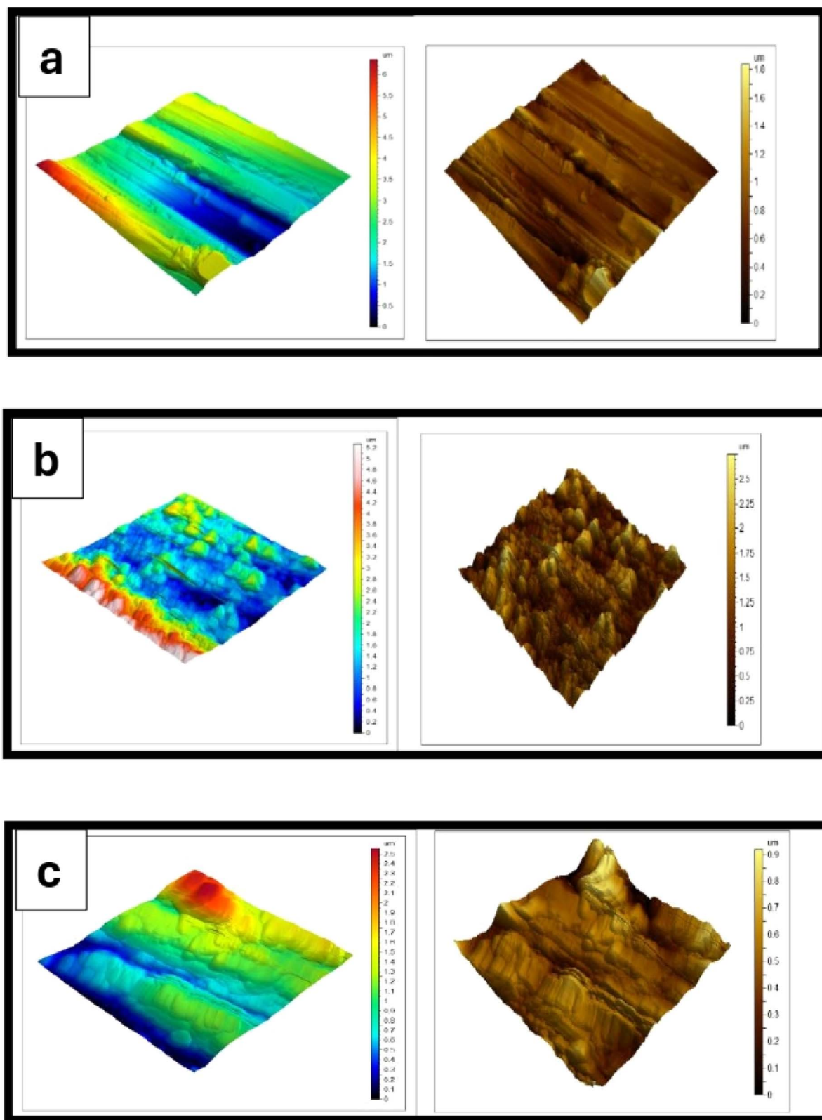
Fig. 8 AFM three-dimensional pictures of LCS (a), LCS after 48 h immersion in a 0.5 mol L -1 HCl without (b) and with (c) 300 ppm of DMIH compound at 298 K.
