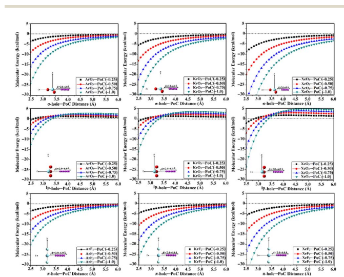
Fig. 3 Curves of molecular energy (in kcal mol -1 ) of ZO_3 \cdots and ZF_2 \cdots PoC systems (where Z = Ar, Kr, and Xe ) at the \sigma -hole-, lp-hole- and \pi -hole \cdots PoC distances ranging from 2.5 to 6.0 Å.
