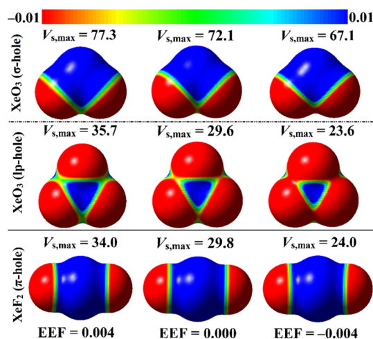
Fig. 7 MEP maps of the optimized \text{XeO}_3 and \text{XeF}_2 monomers under the +0.004, 0.000 and -0.004 au EEF conditions. V_{s,\text{max}} values at the \sigma -/ lp - and \pi -hole sites of the \text{XeO}_3 and \text{XeF}_2 monomers, respectively, are in kcal mol -1 .
