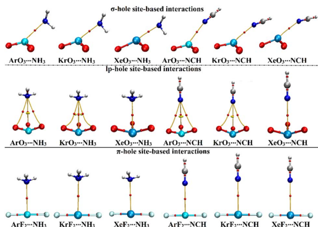
Fig. 5 QTAIM plots of the \sigma -/ lp - and \pi -hole site-based interactions within the ZO_3\cdots and ZF_2\cdots LB complexes, respectively (where Z = \text{Ar} , \text{Kr} , and \text{Xe} ; \text{LB} = \text{NH}_3 and \text{NCH} ).
