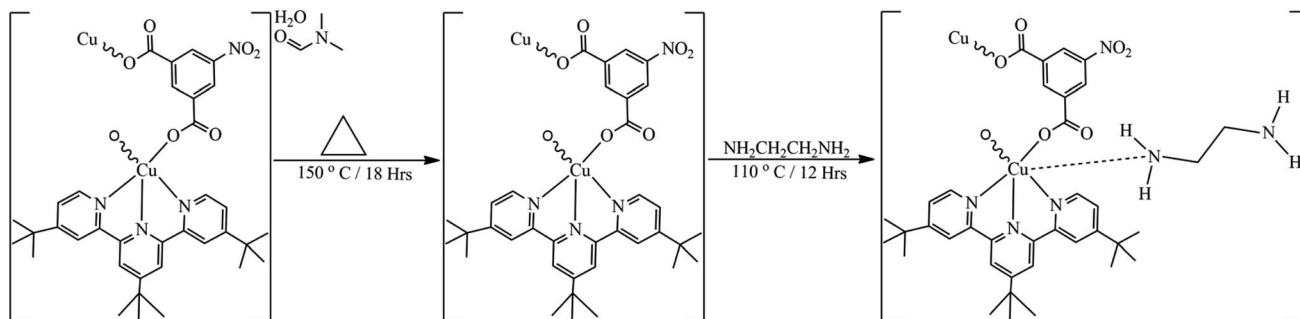
Scheme 2 Amino-functionalization of [Cu(npd)(N 3 ttb)]·(DMF)(H 2 O).
