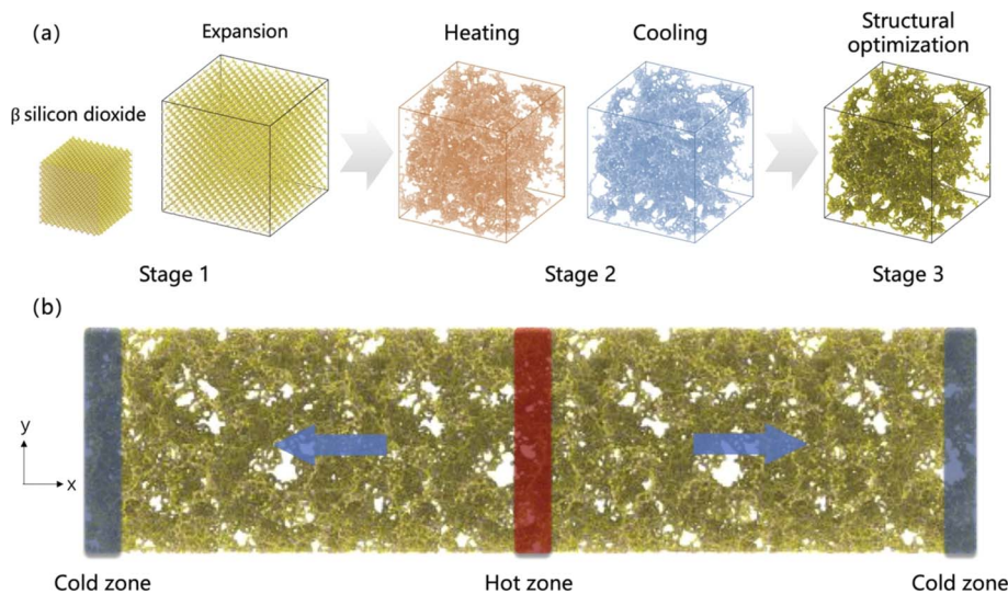
Fig. 1 (a) Three stages of the transformation from β-phase silicon dioxide crystal to SA. (b) Computational model of SA.
