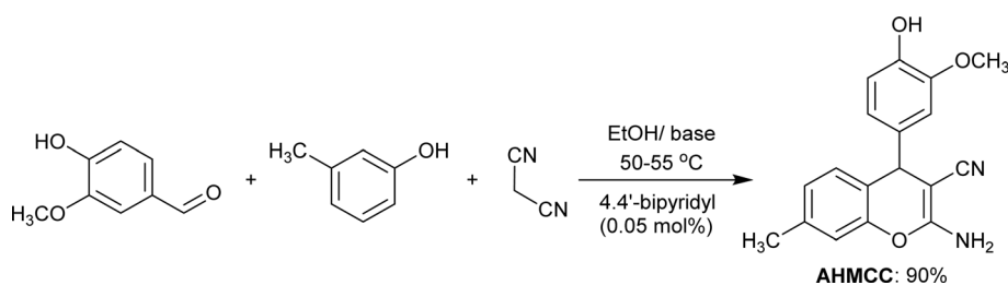
Scheme 1 Synthesis of (AHMCC) inhibitor.
