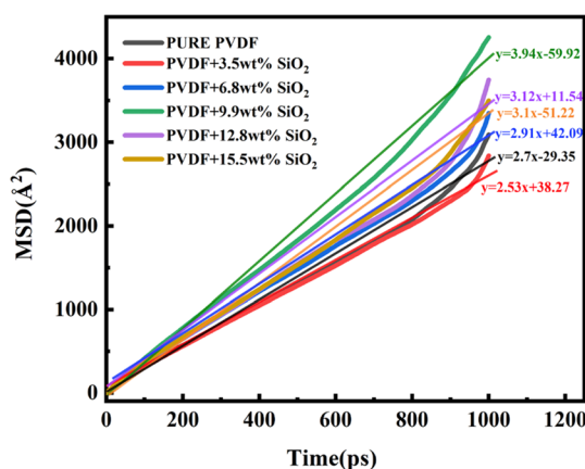
Fig. 8 Change in diffusion coefficient of water.
