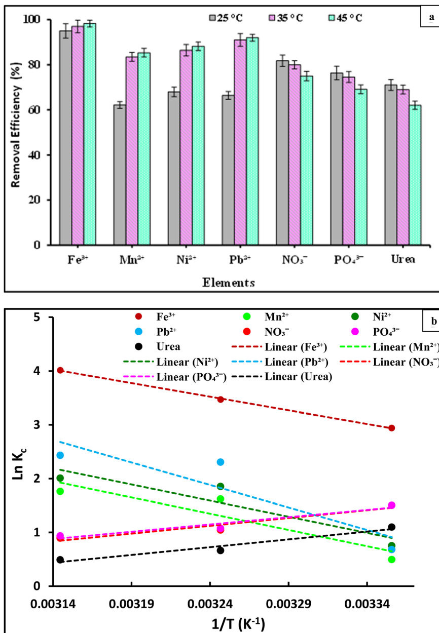
Fig. 8 (a) Effect of temperature; (b) Van't Hoff plot of \ln K_c versus 1/T for adsorption of Fe 3+ , Mn 2+ , Ni 2+ , Pb 2+ , NO 3 - , PO 4 3- , and urea element ions onto the PVC-DAP-0.2 Ag NP membrane, ion concentration 10 mg L -1 , pH = 5–7.2 according to the type of metal ions, time = 120 min., and adsorbent dose is 3 g L -1 .
