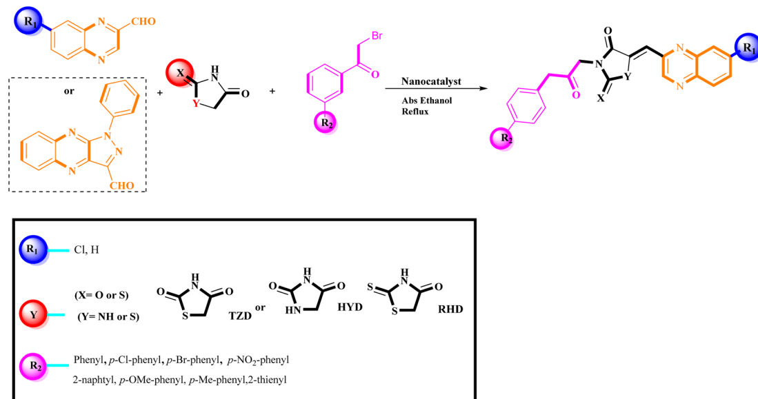
Scheme 3 Synthesis of N -substituted ( Z )-5-arylidene thiazolidine-2,4-dione and related cyclic derivatives by \text{Fe}_3\text{O}_4@\text{CPTMS}@ guanidine- \text{BuSO}_3\text{H} MNPs.
